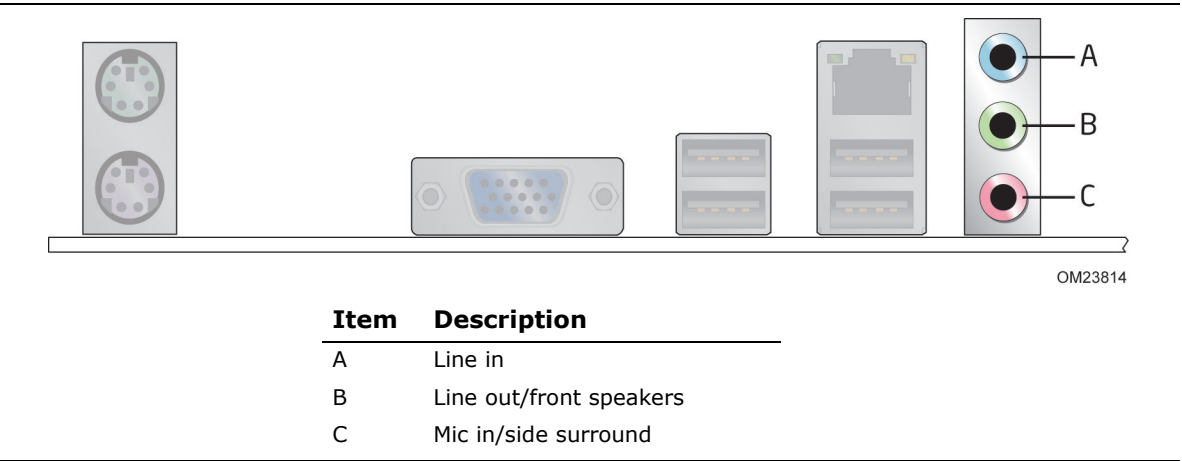
Figure 4. Back Panel Audio Connector Options
