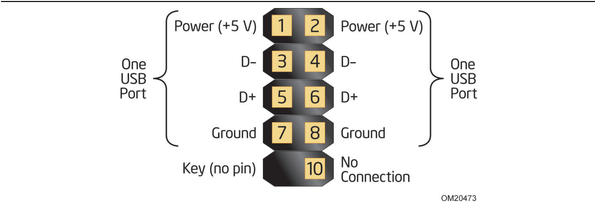
Figure 11. Connection Diagram for the Front Panel USB Header
