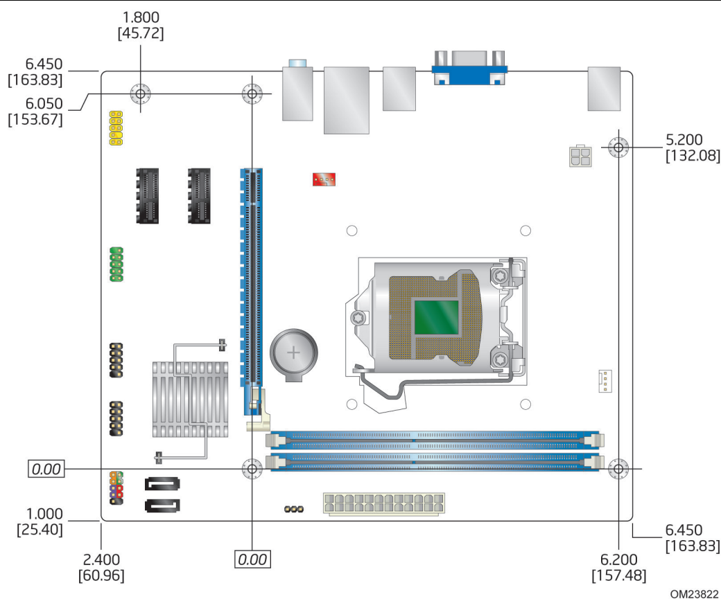
Figure 13. Board Dimensions
