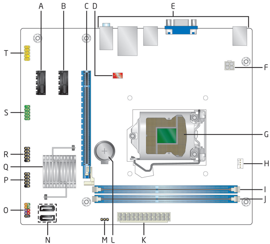
Figure 1. Major Board Components
